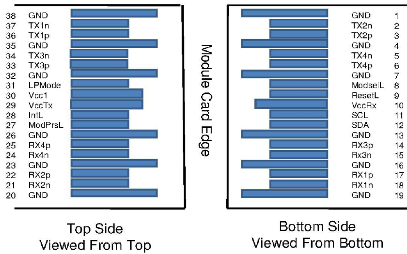
Figure 2 Pin View
