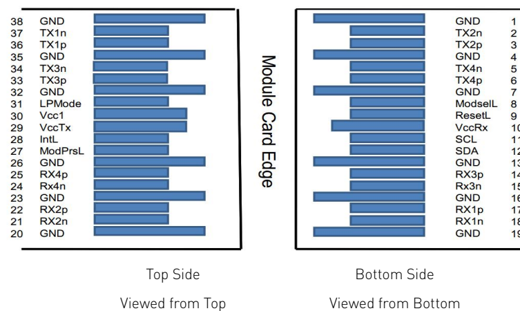
Figure 2 Pin View
