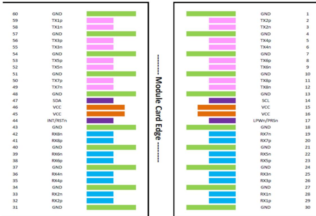
Figure 1 MSA Compliant Connector
