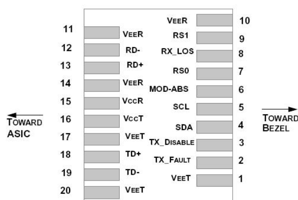
Figure 2 Pin View
