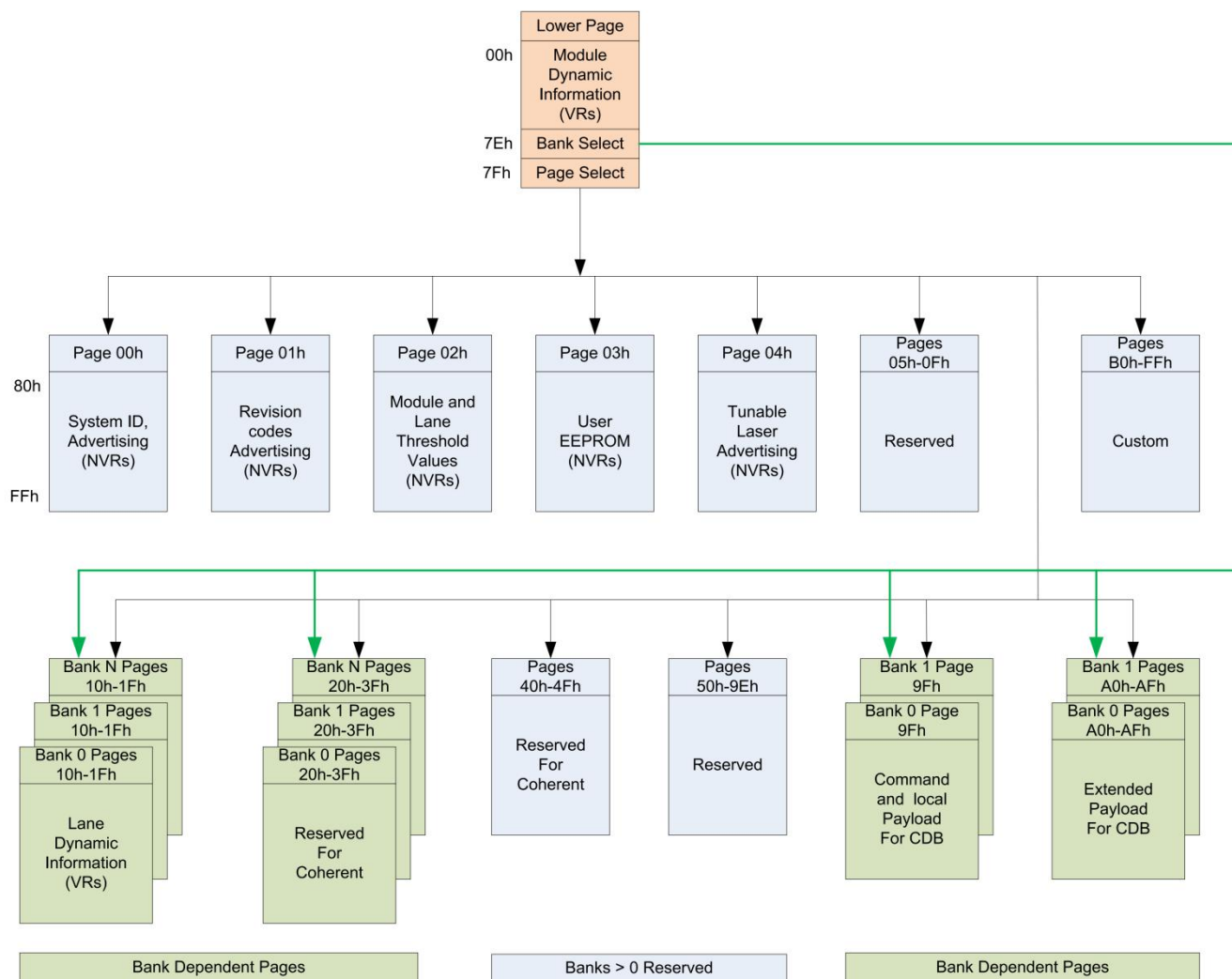
Figure5:Memory map
