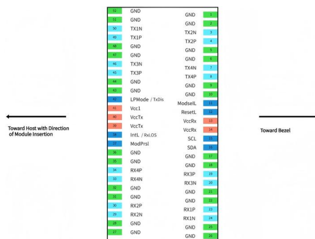
Figure5:Pin view
