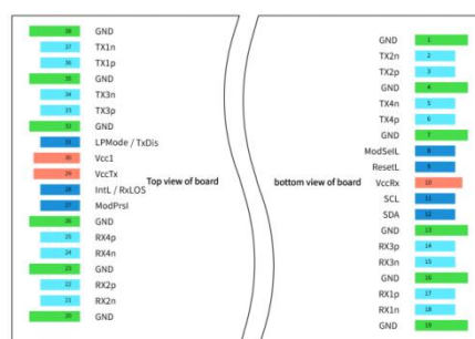
Figure4:QSFP112 Module contact assignment
