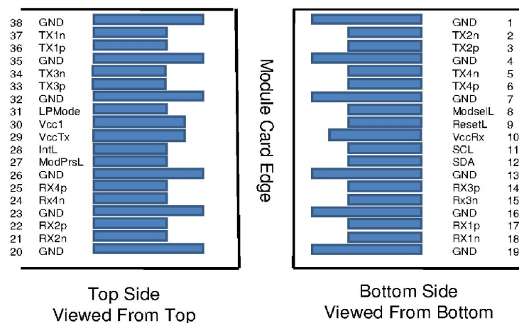
Figure 2 QSFP56 MSA-compliant 38-pin connector
