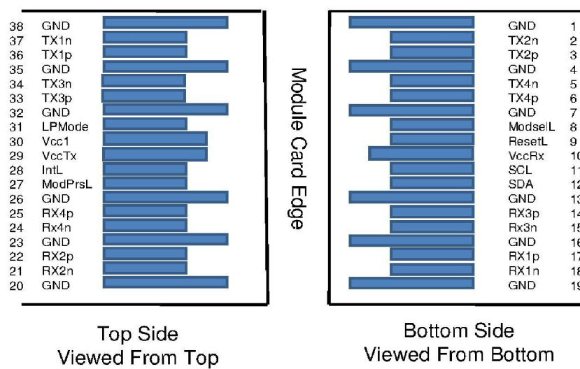
Figure 2 Pin View
