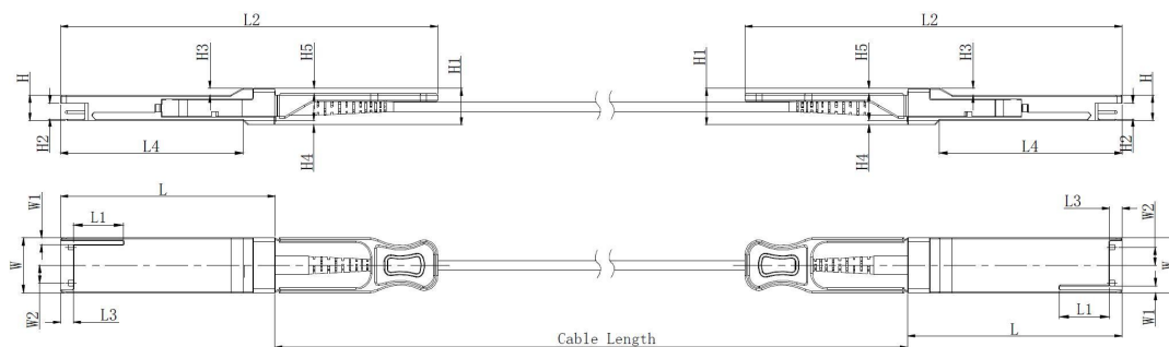
Figure 4 Mechanical Diagram
