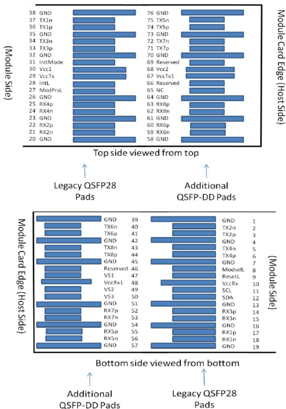
Figure 1 Pin view
