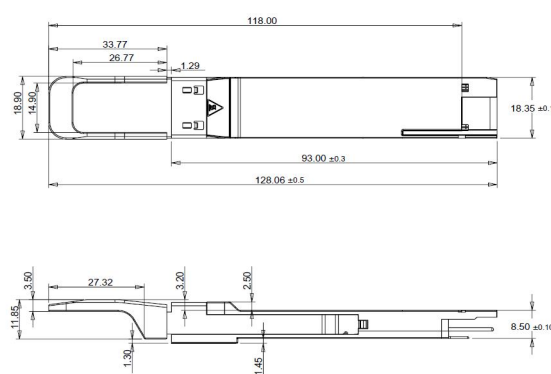
Figure3 Mechanical Outline
