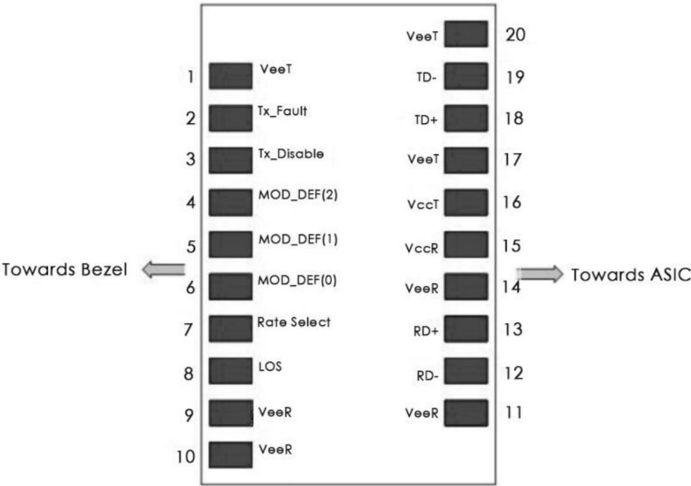
Figure1 Pin view
