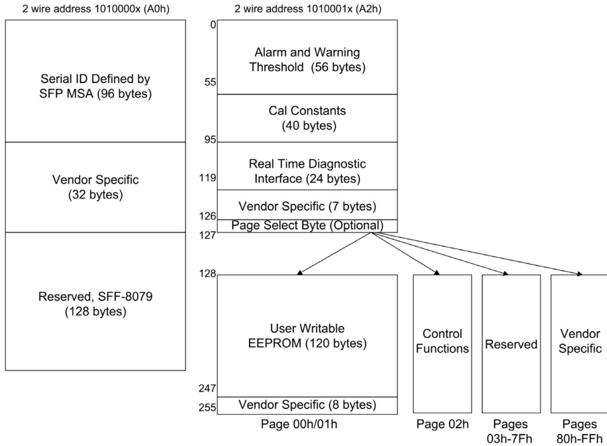
Figure2 Memory map
