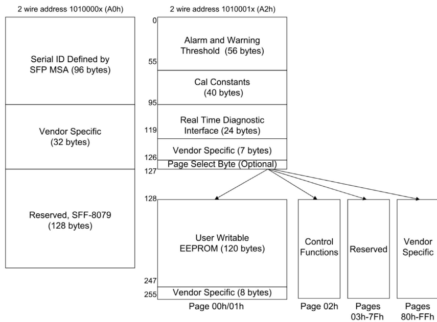
Figure4 Memory map
