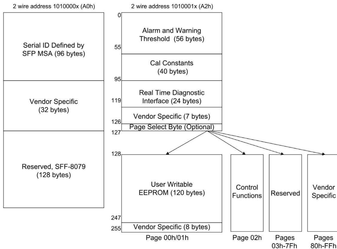
Figure2 Memory map
