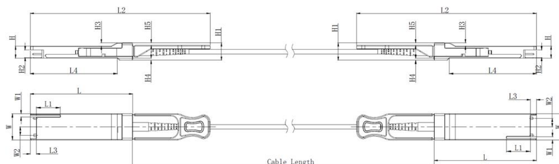
Figure 4 Mechanical Diagram
